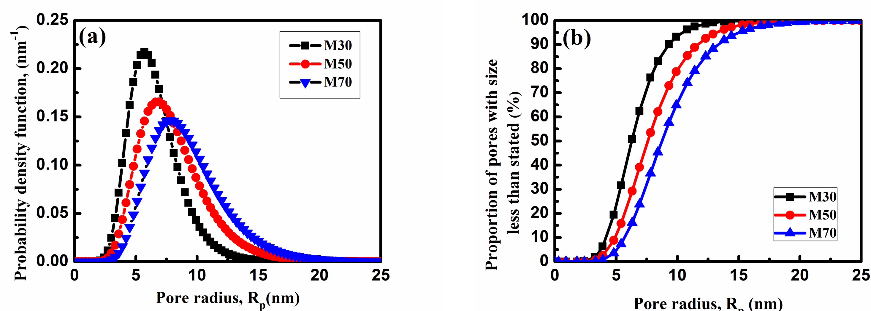
Figure 2. (a) Pore radius distribution curves and (b) cumulative curves.
