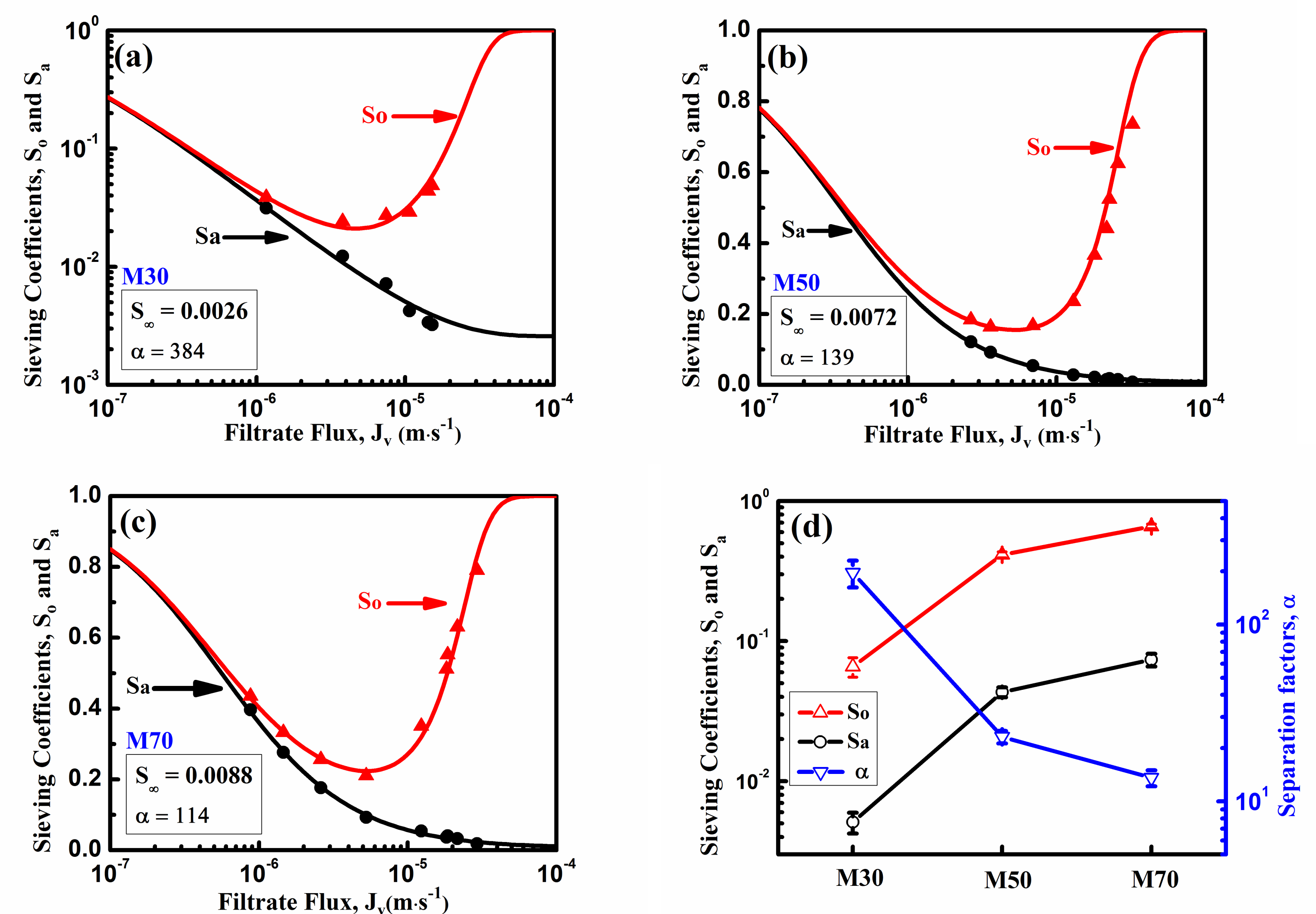
Figure 4. Sieving coefficients and separation factors for PMIA membranes.
