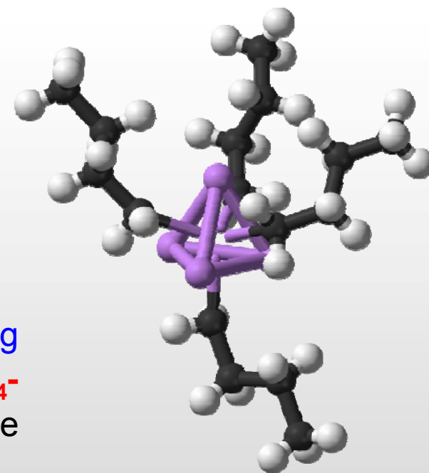
n -Butyllithium
