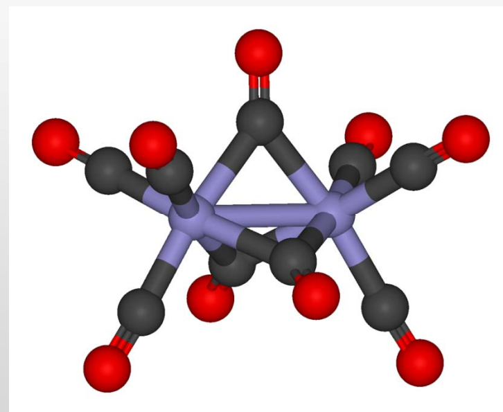
tri- \mu -carbonyl-bis(tricarbonyliron)(Fe-Fe)
