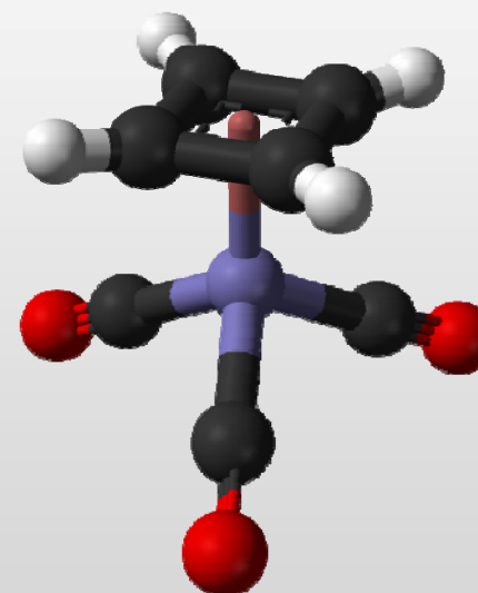
(\text{C}_4\text{H}_4)\text{Fe}(\text{CO})_3
