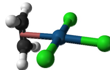
Zeise's salt
